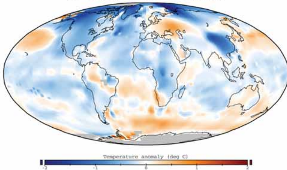
1965-1975 Mean Temperatures vs 1937-1946
