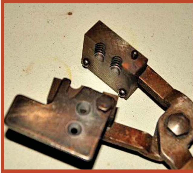
4. This is one type of bullet mold made of steel and made by RCBS. (Author Photo)
