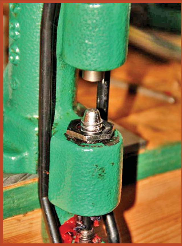
8. This is how the bullet is placed in the machine. The handle is pulled and the bullet is pressed down into a die forming it to the proper diameter and injecting the lube.
